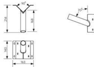
LEDStreetlight Wall Bracket
