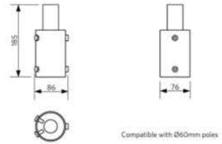
LEDStreetlight Pole Top Adapter 60
