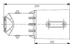
Pole Adapter-Roadlight-76mm
