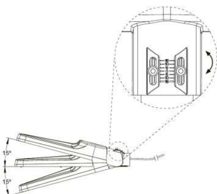
LEDRoadlight Tilting
