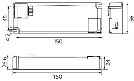
LEDPanelRc-Mo Driver On/Off
