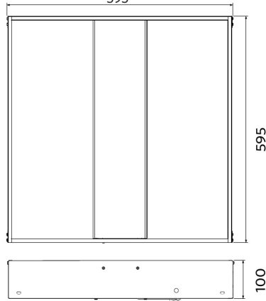
LEDPanelRc-Mo Driver Dim
