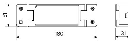
LEDPanelRc-Mo Driver Dim
