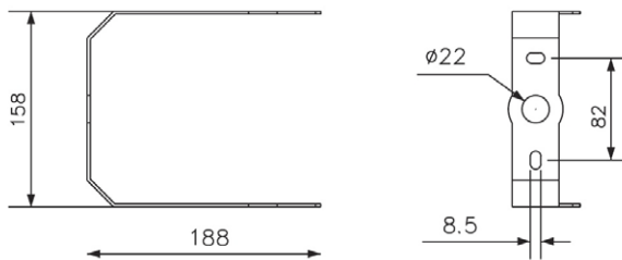
LEDHighbay-P4 Bracket-D330
