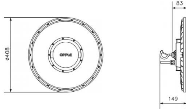
LEDHighbay-P4 Bracket-D420
