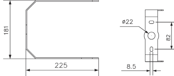
LEDHighbay-P4 Bracket-D420
