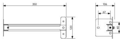
LEDflood-E-Re150-Bracket
