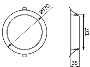
LEDDownlightCo-E Rd150
