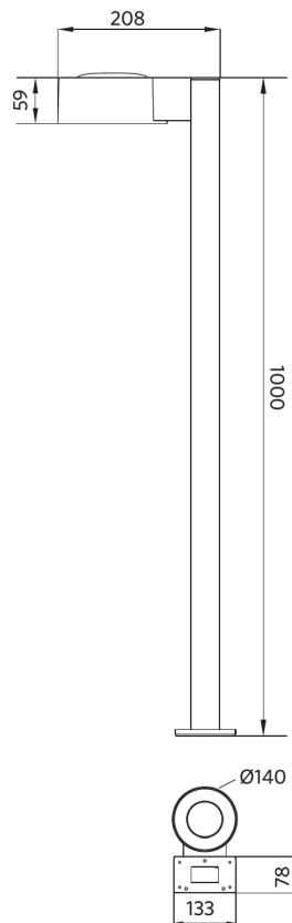
LEDBollard-Luke-E L1000-8W
